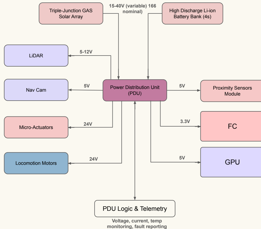
DRONE POWER ARCHITECTURE
