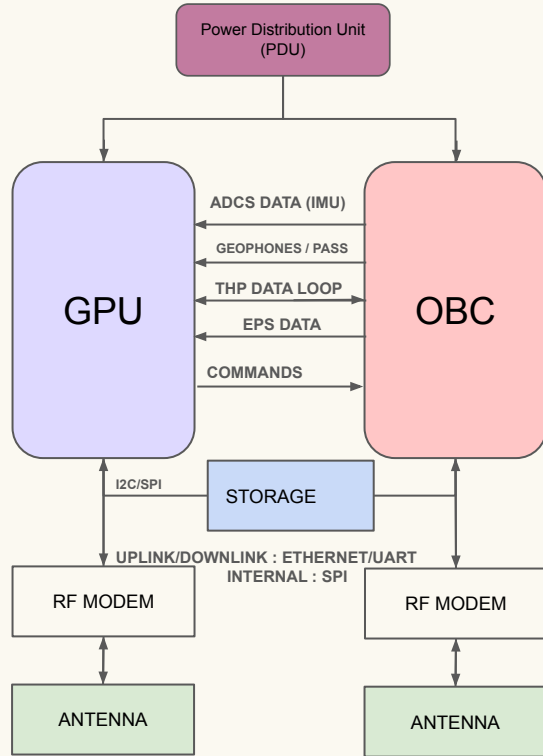
OBDH SYSTEM ARCHITECTURE
